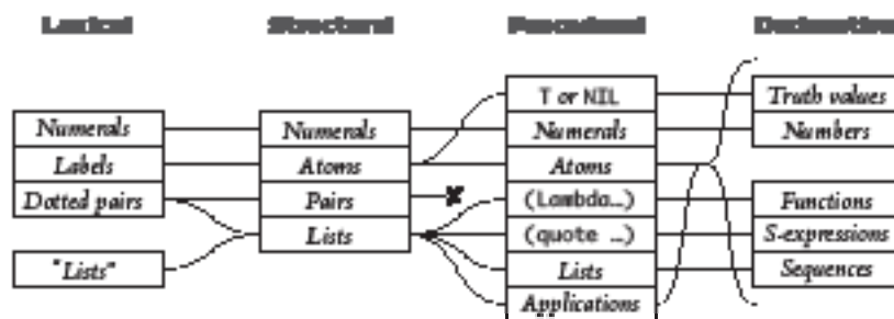
Figure 9 — The Category Structure of Lisp 1.5
