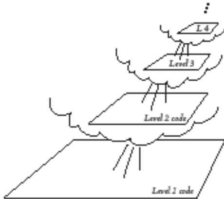
Figure 15 — The 3Lisp Reflective Tower
