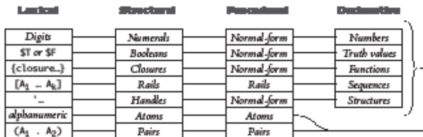
Figure 10 — The Category Structure of 2Lisp
